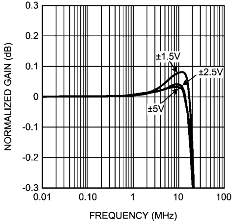
±0.1 dB Gain Flatness for Various Supplies
